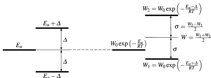
Fig. 1. Scheme of the transition probability distribution.
