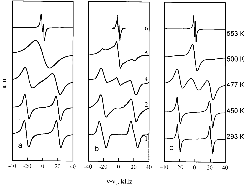
Fig. 2. The temperature dependence of the ^1\text{H} NMR spectrum of natrolite for the case when the vector \mathbf{B}_0 lies in [110] direction: (a) theoretical NMR spectra obtained for the model of homogeneous diffusion of water molecules with the activation energy E_a = 73 kJ/mole; (b) experimental NMR spectra; (c) theoretical NMR spectra obtained for the non-Markov model of motion ( E_a = 73 kJ/mole and \Delta = 4.2 kJ/mole).
